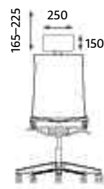
NAVIGO UPH HRUA LP11 RTS TS25 (ST44) ESH Gewicht | Poids: 15.15 kg (15.40 kg) NAVIGO MESH/MESH PLUS Gewicht | Poids: 14.65 kg (14.90 kg)
