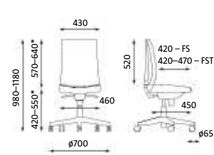
NAVIGO UPH FS RTS TS25 (ST44) ESH Gewicht | Poids: 14.65 kg (14.90 kg) NAVIGO MESH/MESH PLUS Gewicht | Poids: 14.15 kg (14.40 kg)
