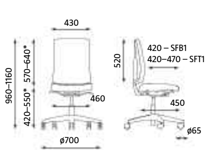
NAVIGO UPH SFB1 RTS TS25 (ST44) ESH Gewicht | Poids: 14.80 kg (15.05 kg) NAVIGO MESH/MESH PLUS Gewicht | Poids: 14.30 kg (14.55 kg)
