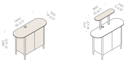
en_Pantry it_Pantry fr_Pantry en_Shelf with or without LED light it_Mensola con o senza LED fr_Étagère avec ou sans LED
