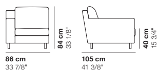
cod. 5109 / left element 86
